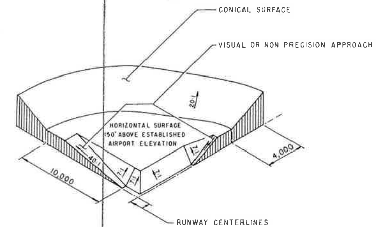
ISOMETRIC VIEW No Scale
